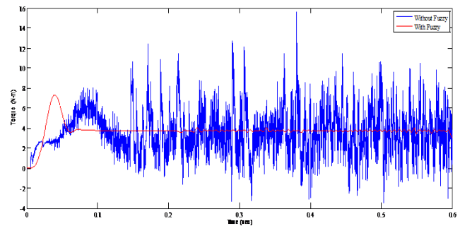
Fig. 9: Comparison of Electromagnetics Torques of IM for only FLC replacing FHB with THB and Without Fuzzy Logic Controller
